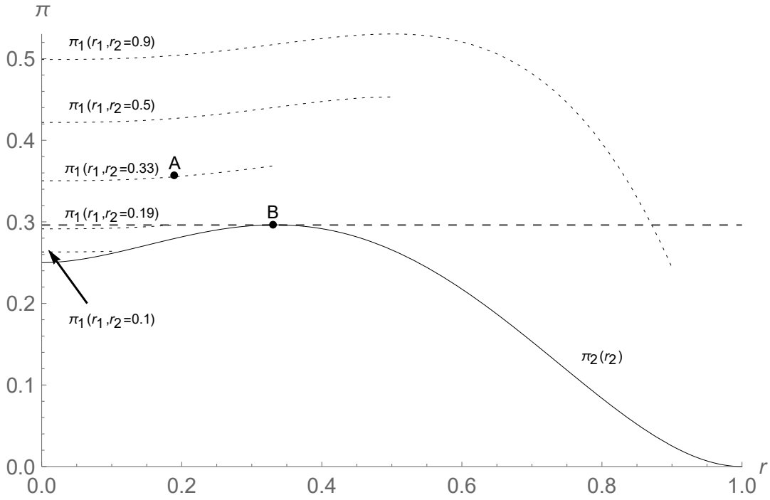
Figure 1: Equilibrium in reserve prices (points A and B) when n = 3 and v_i \sim U[0, 1] .
